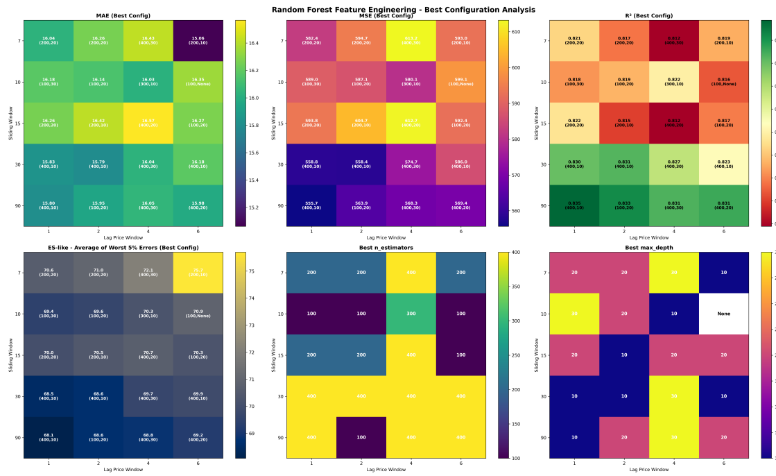
Fig. 4.15. Feature Engineering Random Forest Metrics Distribution
